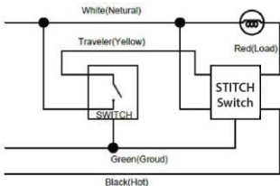
Wiring Method 1
