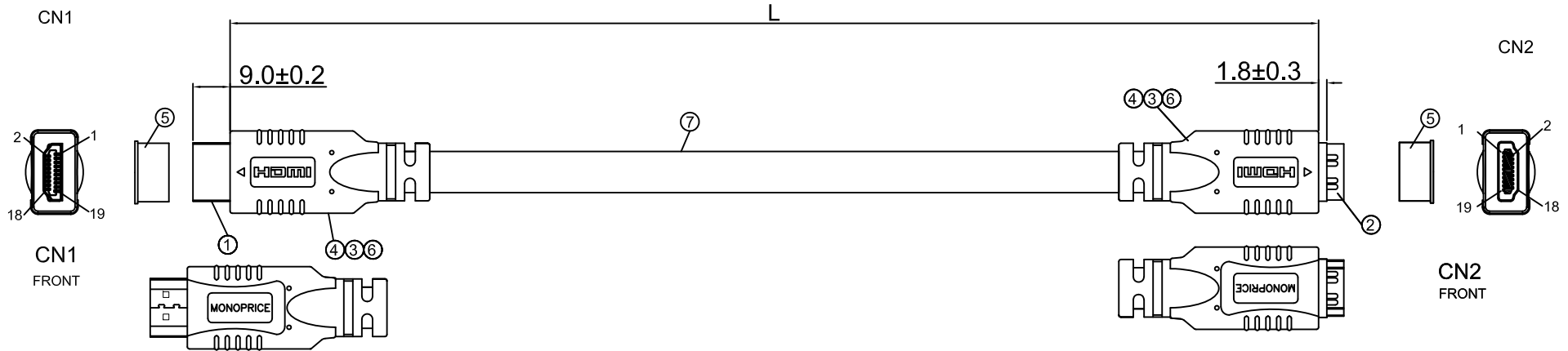
HDMI 19P/M MOLDING TYPE
