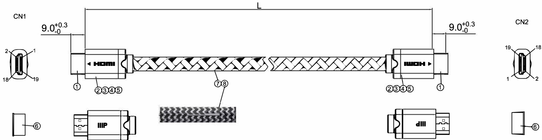
HDMI 19P/M MOLDING TYPE
