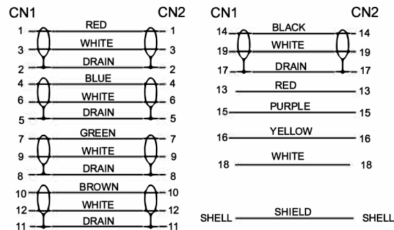
HDMI 19P/M MOLDING TYPE
