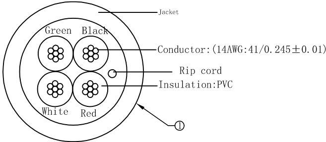
CROSS-SECTION
