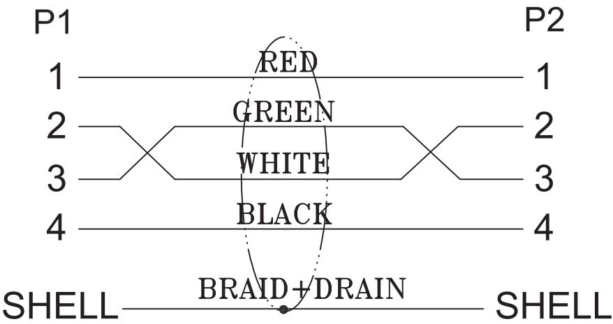
PIN OUT
