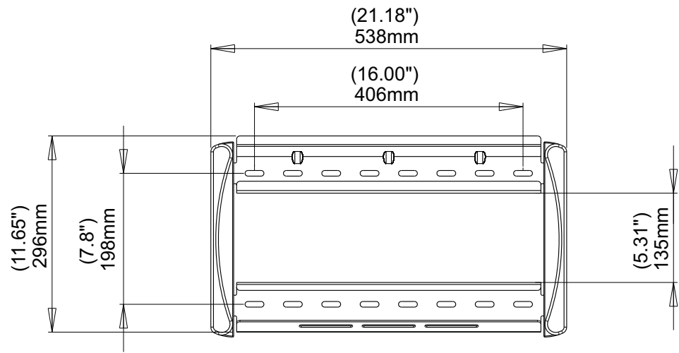
WALL PLATE DETAILS
