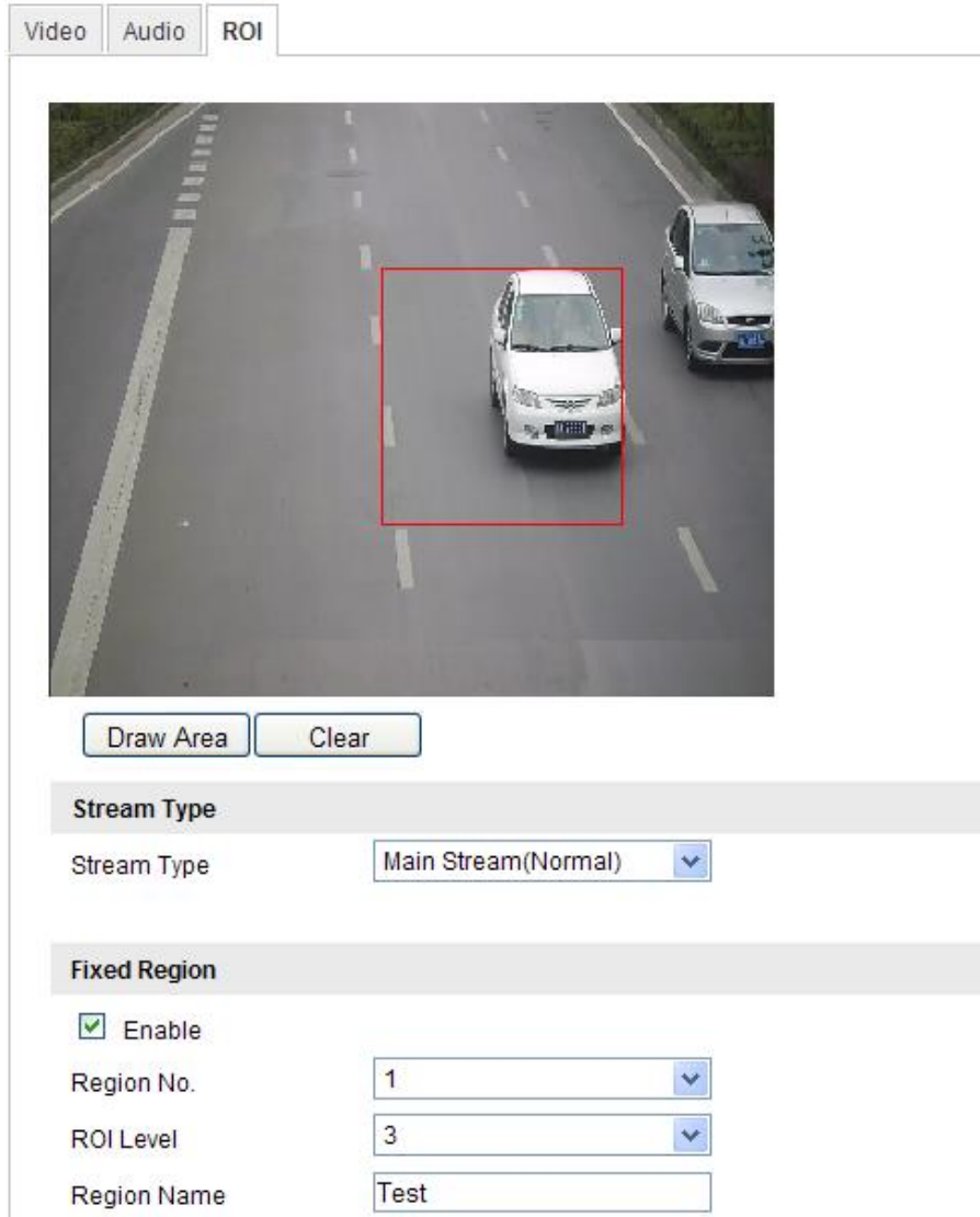
Figure 6-24 Region of Interest Settings
