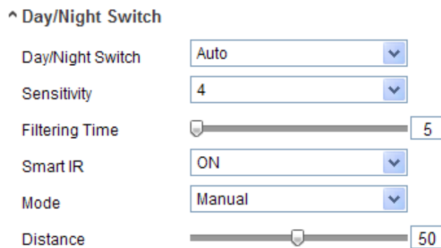
Figure 6-26 Day/Night Switch
