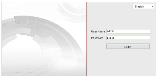
Figure 4-1 Login Interface
