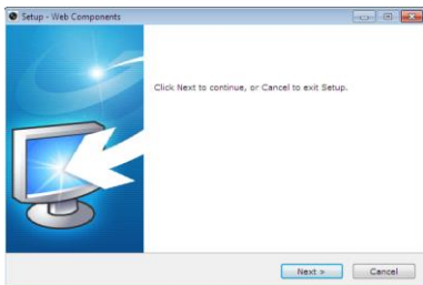
Figure 4-3 Install Plug-in(1)
