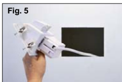
Figure 5 Now use the four screws provided to secure the electrical outlet box to the mounting studs on the backside of the Mid-Size Plate.
