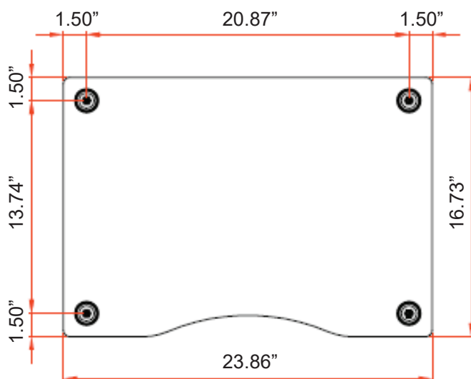
Top view drawing
