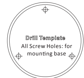
Figure 2-1 Drill Template
