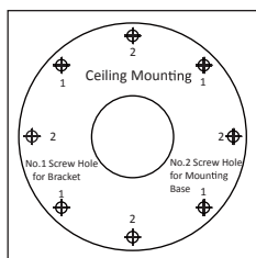
Figure 2-4 Drill Template
