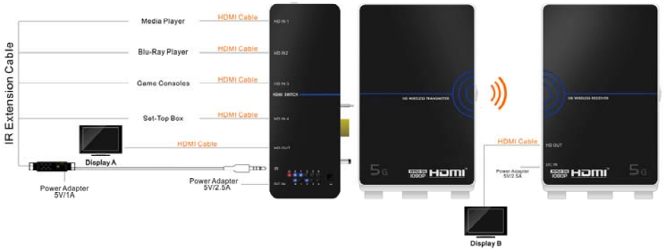
Image 6 Installation Diagram for Matrix Display
