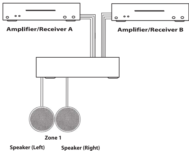
Figure 1: Wiring Diagram
