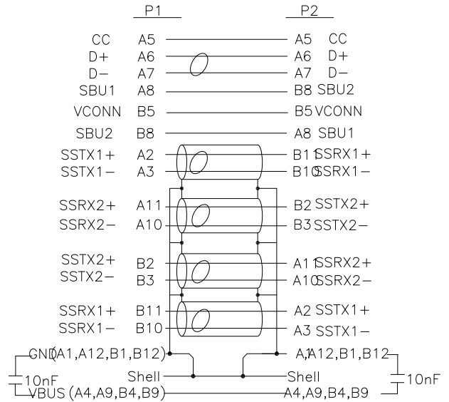
Pin Assignment
