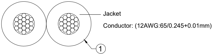
CROSS-SECTION
