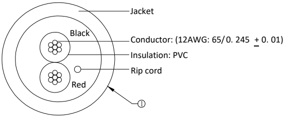
Cross Section
