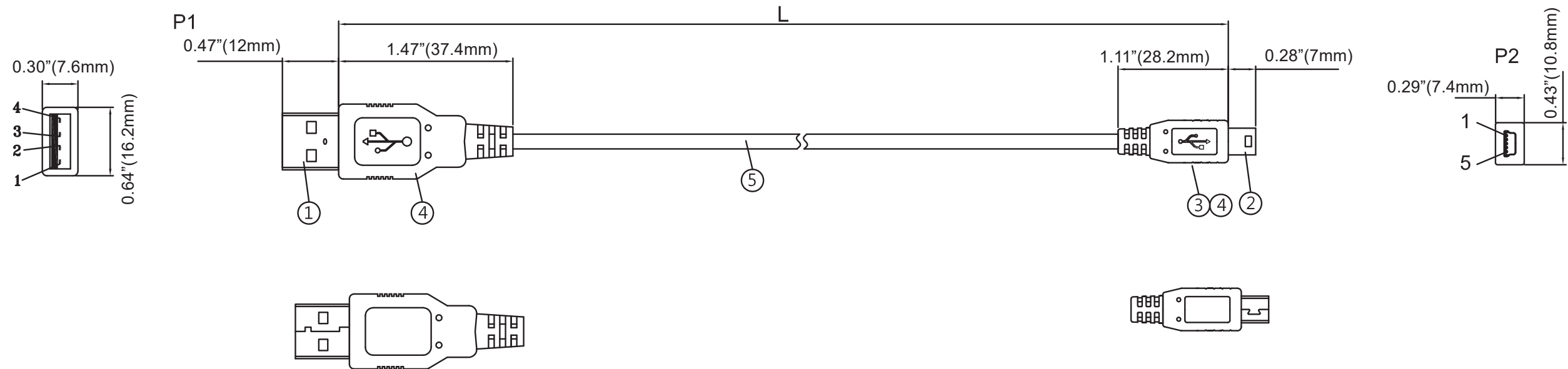
USB A/M MOLDING TYPE
