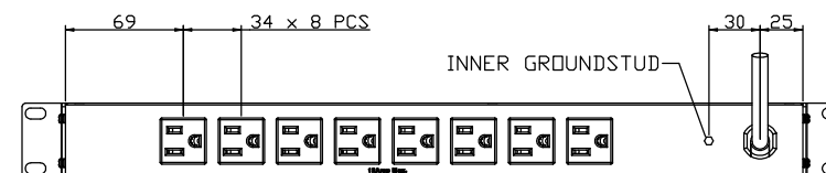
< Rear View >
