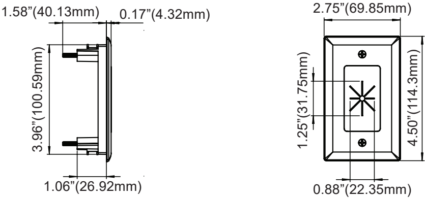
48599 (Black) 1-Gang Cable Plate with Flexible Opening
