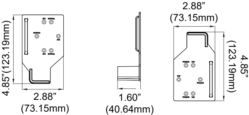
Bracket Dimensions
