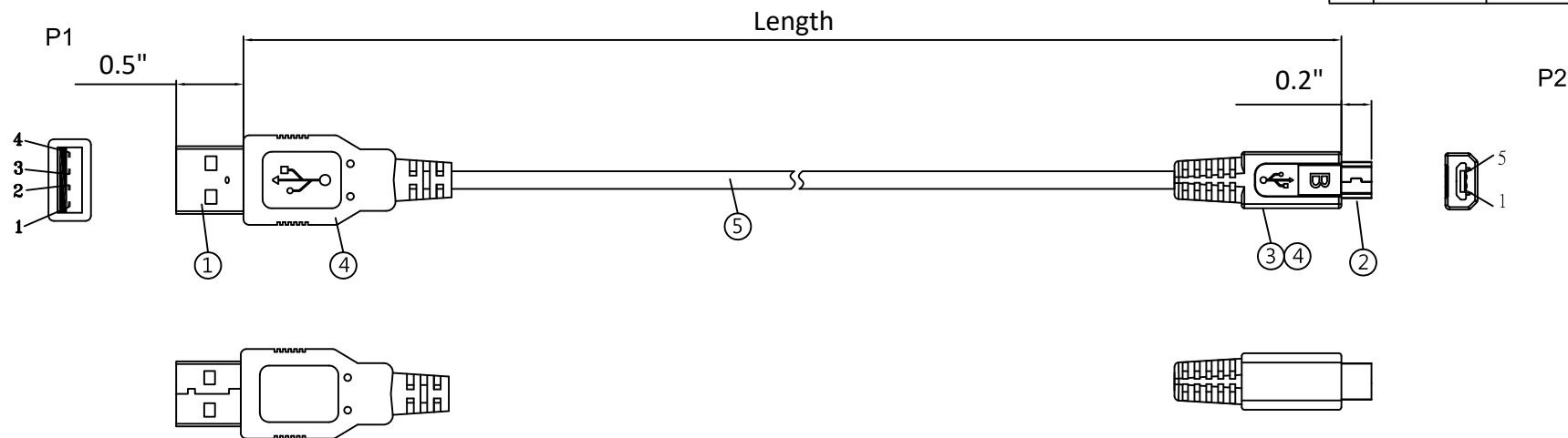
USB A/M MOLDING TYPE
