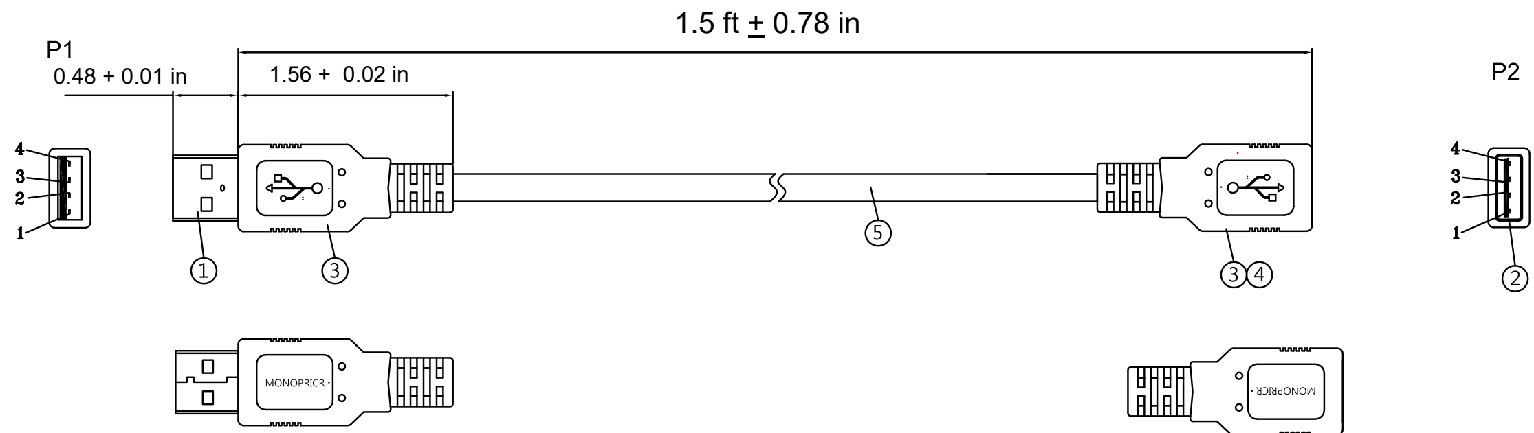
USB A/M MOLDING TYPE
