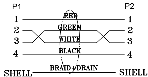
PIN OUT
