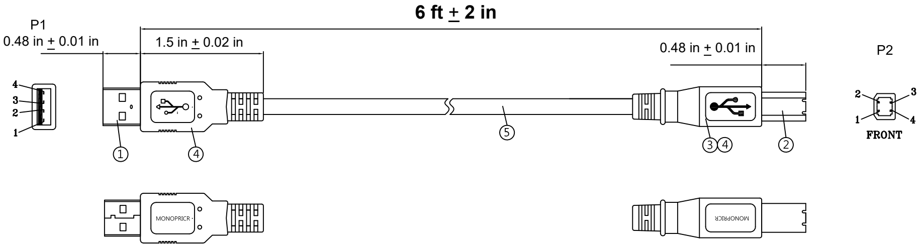
USB A/M MOLDING TYPE
