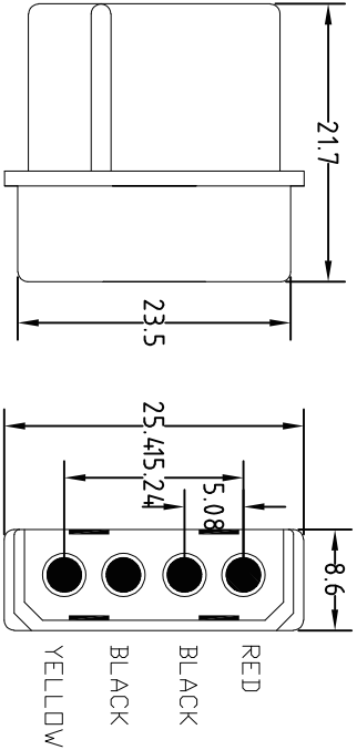
4P housing male connector
